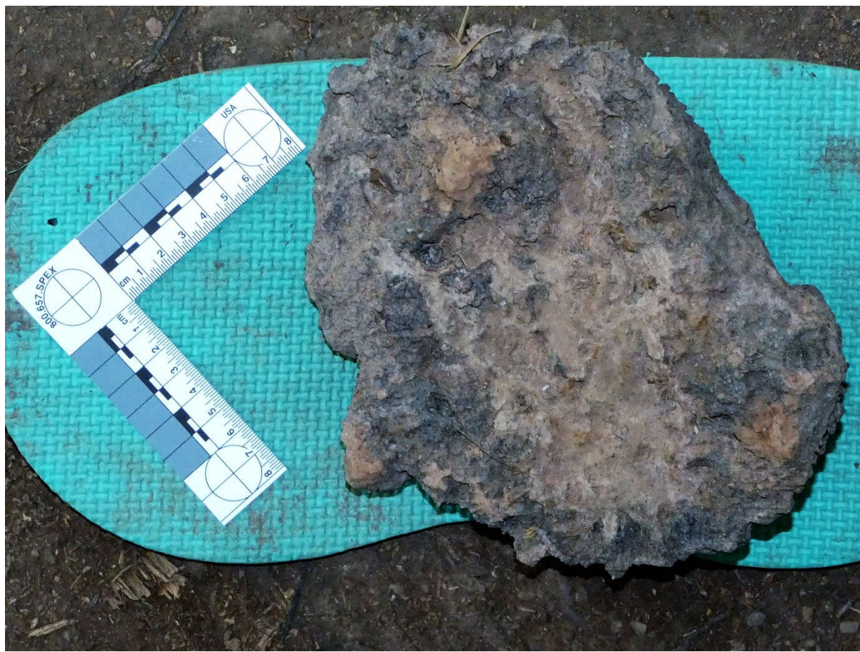
Fig. 10 Example of furnace bottom slag
